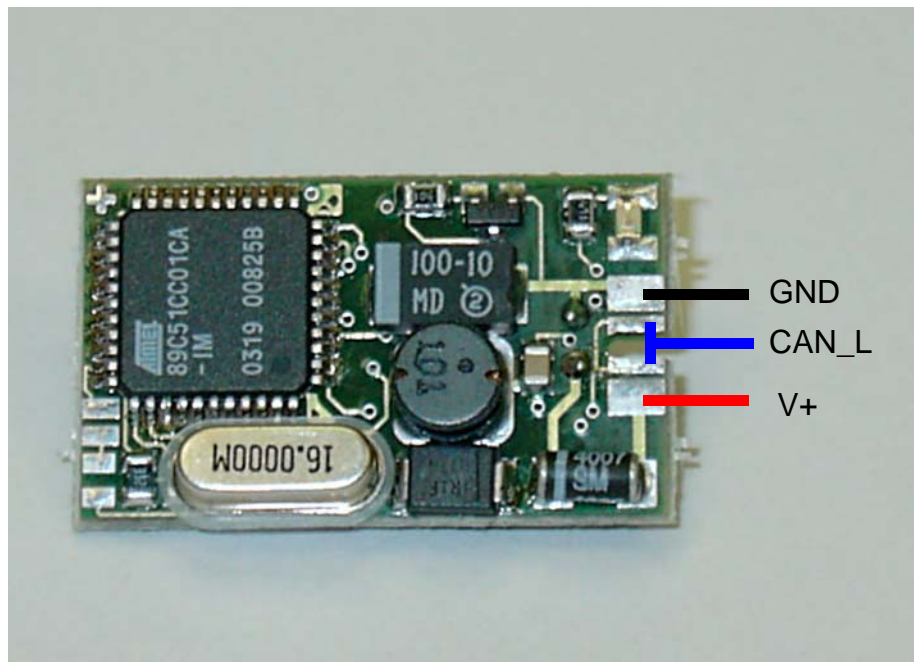
Fig. 6: Connecting of power supply and CAN (top side view)
